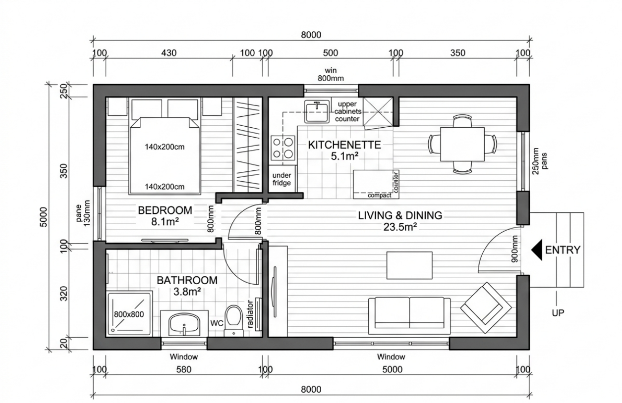
MODERN COMPACT HOUSE 40 sqm - FLOOR PLAN
